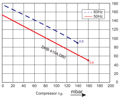
Compressor selection diagram curve
